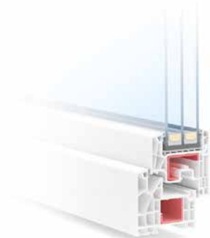
6 chambers depth of frame 82 mm
